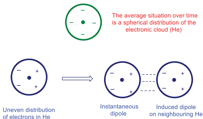
Fig. 5.14: London dispersion forces.
