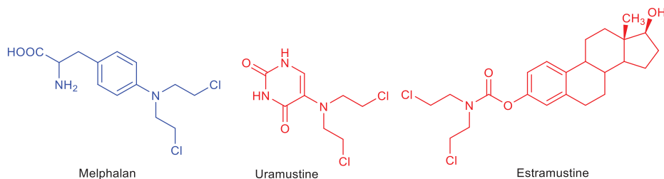
Fig. 4.9: Carrier groups increase cell or tissue selectivity of the drug.
