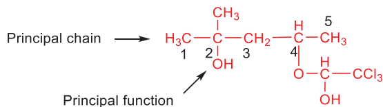
2-Methyl-4-(2,2,2-trichloro-1-hydroxyethoxy)pentan-2-ol
