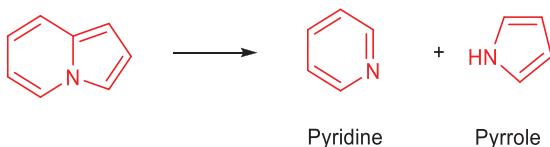
Fig. 2.36: Separation of a bicyclic system into its components, when the heteroatom is at the confluence of two rings.
