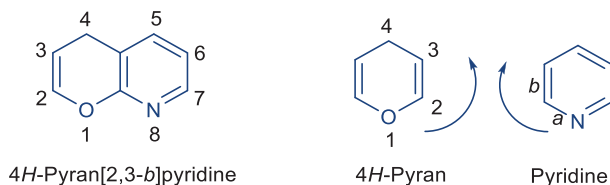
Fig. 2.37: Naming and numbering a condensed bis-heterocycle, having a nitrogen atom.
