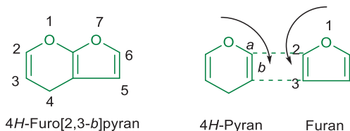
Fig. 2.40: The largest ring is the main component for a condensed bis-heterocycle with the same heteroatom.
