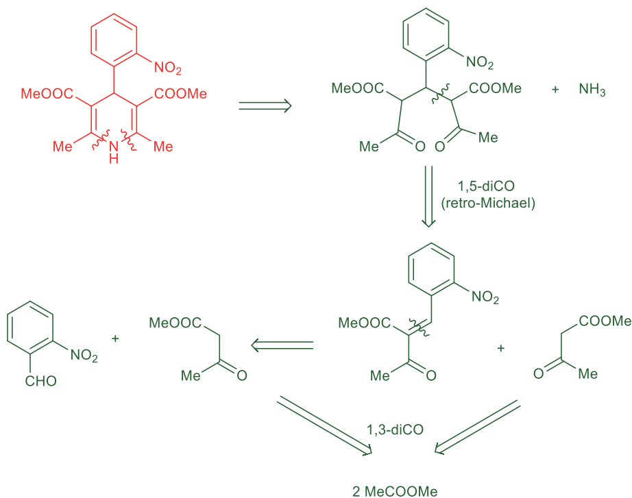
Scheme 9.3: Retrosynthesis of nifedipine.
