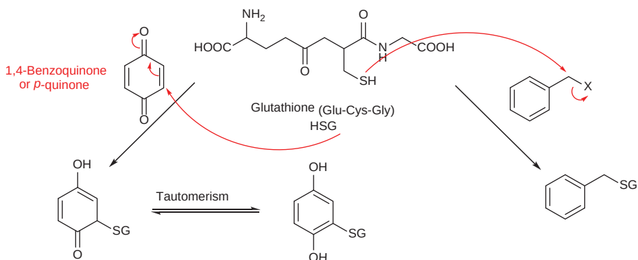
Fig. 7.13: Reaction of GSH with double activated bonds and benzyl halides.
