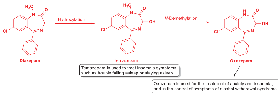
Fig. 7.6: Metabolism of diazepam.
