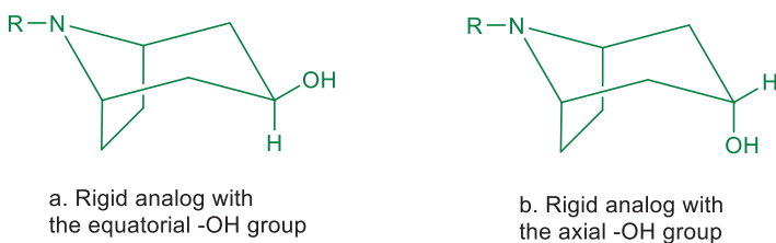
Fig. 5.25: Chair conformations of 4-(4-hydroxypiperidino)-4'-fluorobutyrophenone.
