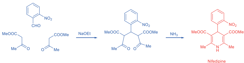
Scheme 9.4: Synthesis of nifedipine.
