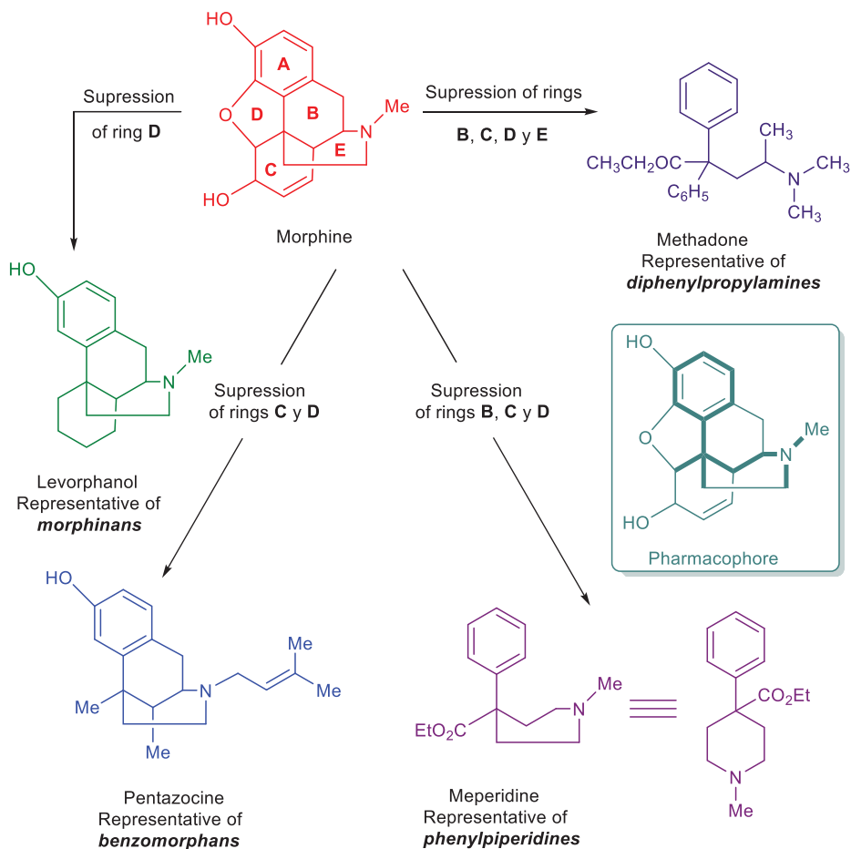
Fig. 4.30: Simplification of the prototype (disjunctive replication) morphine.
