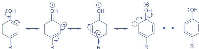
Fig. 6.8: Effects of the phenol group at meta - and para -positions.
