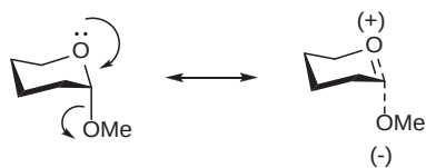
Fig. 7.11: One interpretation of the anomeric effect.
