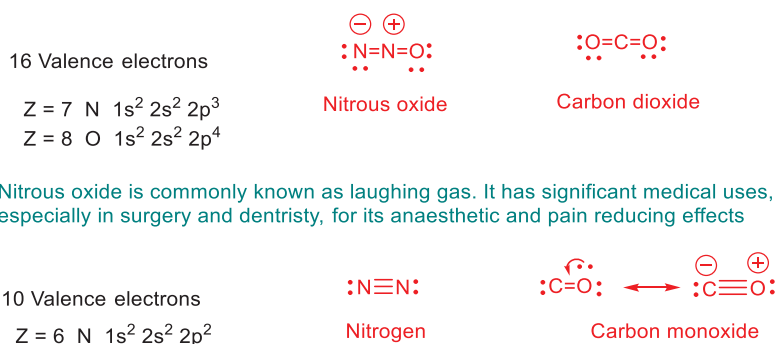
Fig. 4.18: Examples of isosteric molecules.
