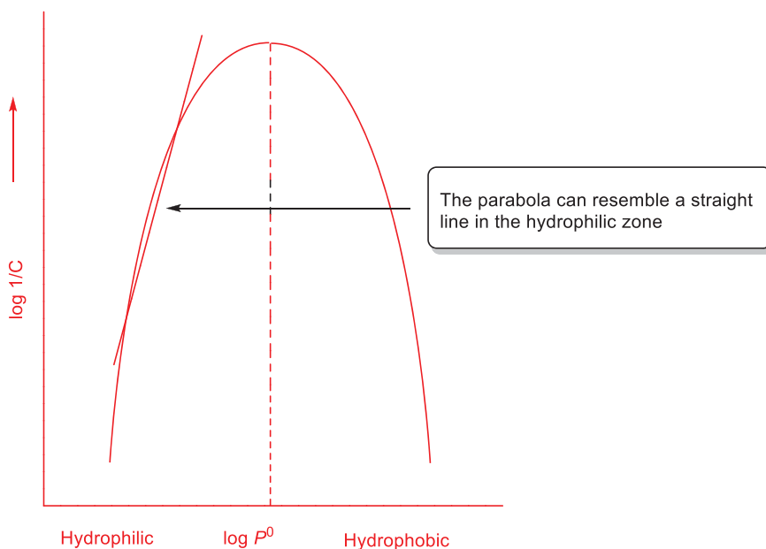
Fig. 6.14: Parabolic dependence of the biological response against the logarithm of the partition coefficient n -octanol/water.
