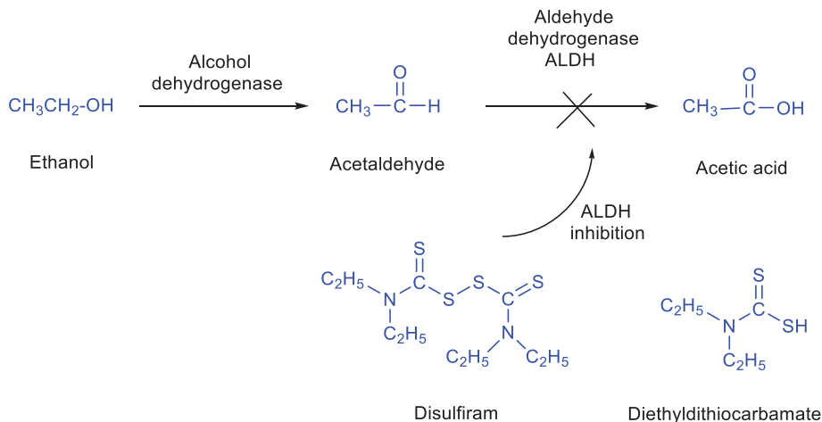
Fig. 3.7: Inhibition of aldehyde dehydrogenase (ALDH) by disulfiram.
