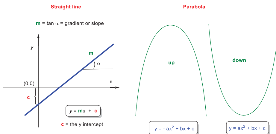
Fig. 6.1: Linear and second-degree equations.
