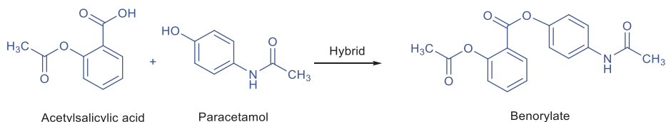
Fig. 4.32: Molecular combination of the prototypes (disjunctive replication) acetylsalicylic acid and paracetamol.
