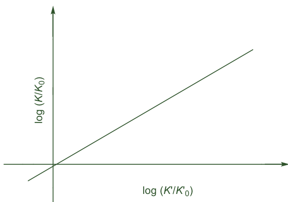
Fig. 6.2: Correlation between the dissociation constants of unsubstituted and substituted benzoic acids (abscissa axis) and those of phenylacetic acids (ordinate axis) with the same substitution patterns ( meta and para ).
