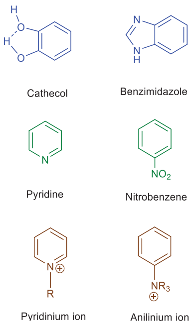
Fig. 4.22: Bioisosteres based on analogous electronic distribution and polarizability.
