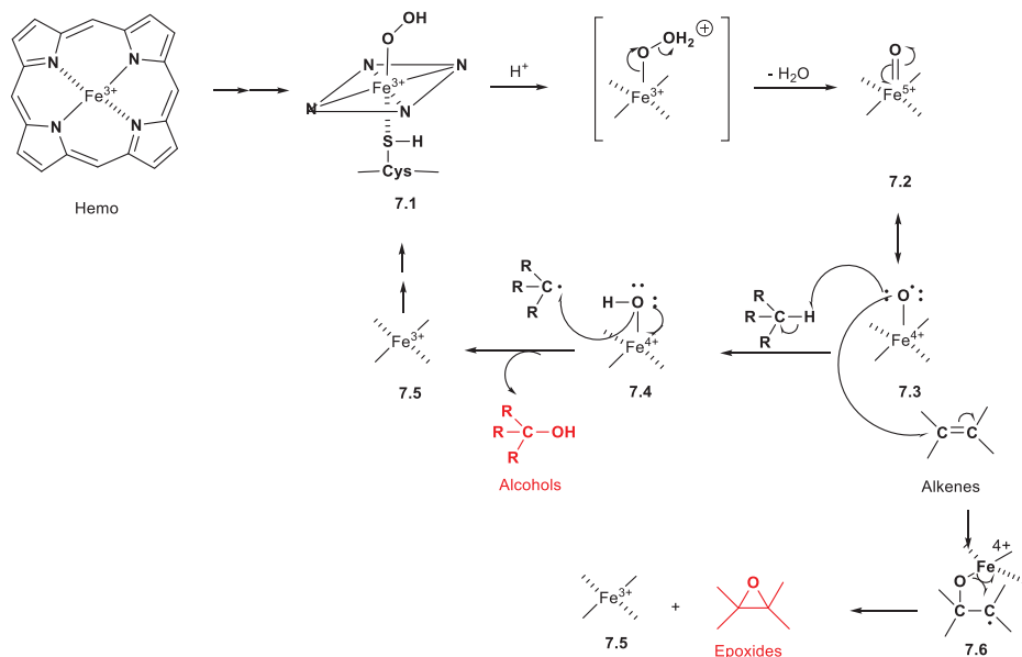
Scheme 7.1: Mechanisms of oxidation reactions of alkanes, alkenes, and arenes catalyzed by cytochrome P450.
