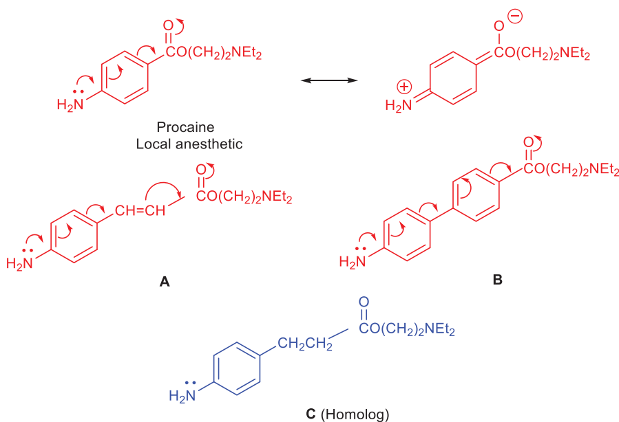
Fig. 4.11: Active vinylogous ( A and B ) of procaine; C is an inactive homolog of procaine.
