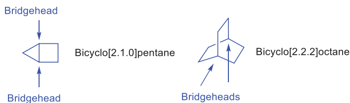
Fig. 2.18: Bridge systems.
