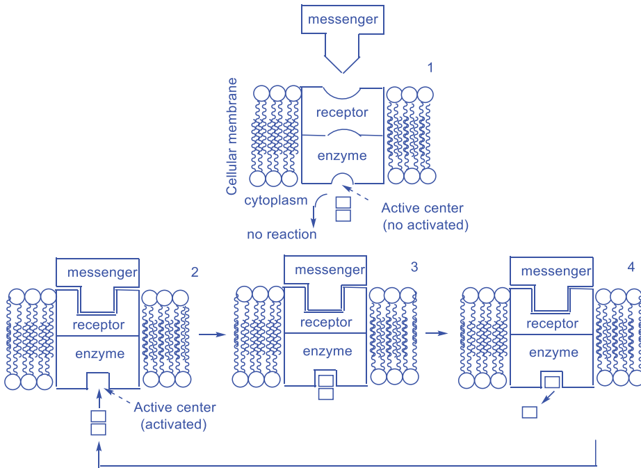
Fig. 5.3: Mechanism of activation of an enzymatic system associated with a membrane receptor: (1) rest state; (2) the enzyme acquires a productive conformation by interaction of the messenger with the receptor; (3) and (4): enzymatic process and return to (2).
