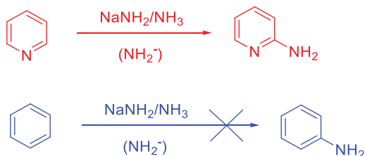
Fig. 4.25: Reactivity of pyridine against \text{S}_{\text{N}}\text{Ar} .
