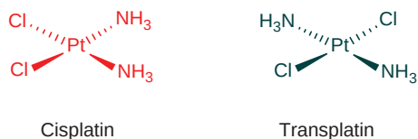
Fig. 5.31: Cisplatin and transplatin.
