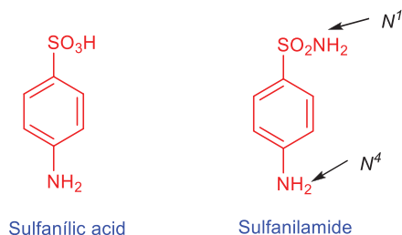
Fig. 2.10: Sulfanilic acid and sulfanilamide.
