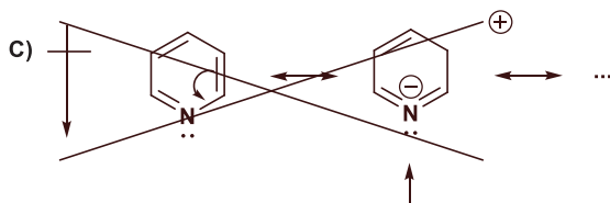
Fig. 4.24: Several possibilities for the electronic distribution of pyridine, although only one is the real one.
