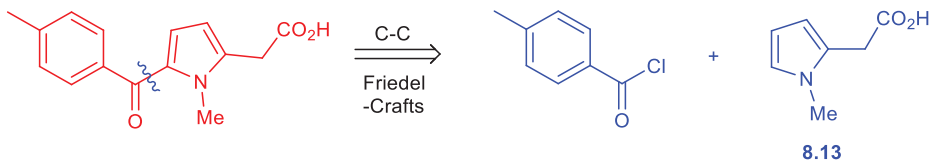
Scheme 8.24: Disconnection of tolmetin.
