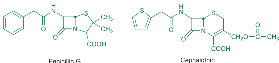
Fig. 2.22: A penicillin and a cephalosporin.
