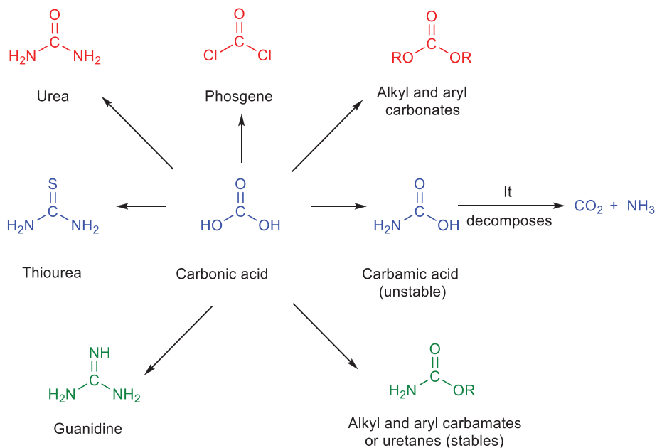
Fig. 2.28: Carbonic acid derivatives.
