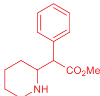
(h) Methylphenidate
