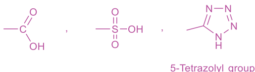
Fig. 4.28: Groups with similar acidity.
