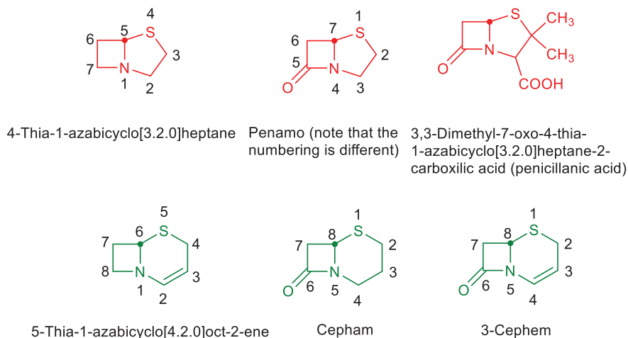
Fig. 2.23: Several possibilities of naming penicillins and cephalosporins.
