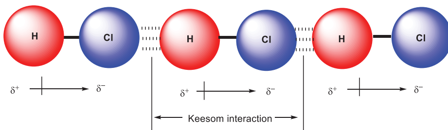
Fig. 5.15: Keesom orientation forces.
