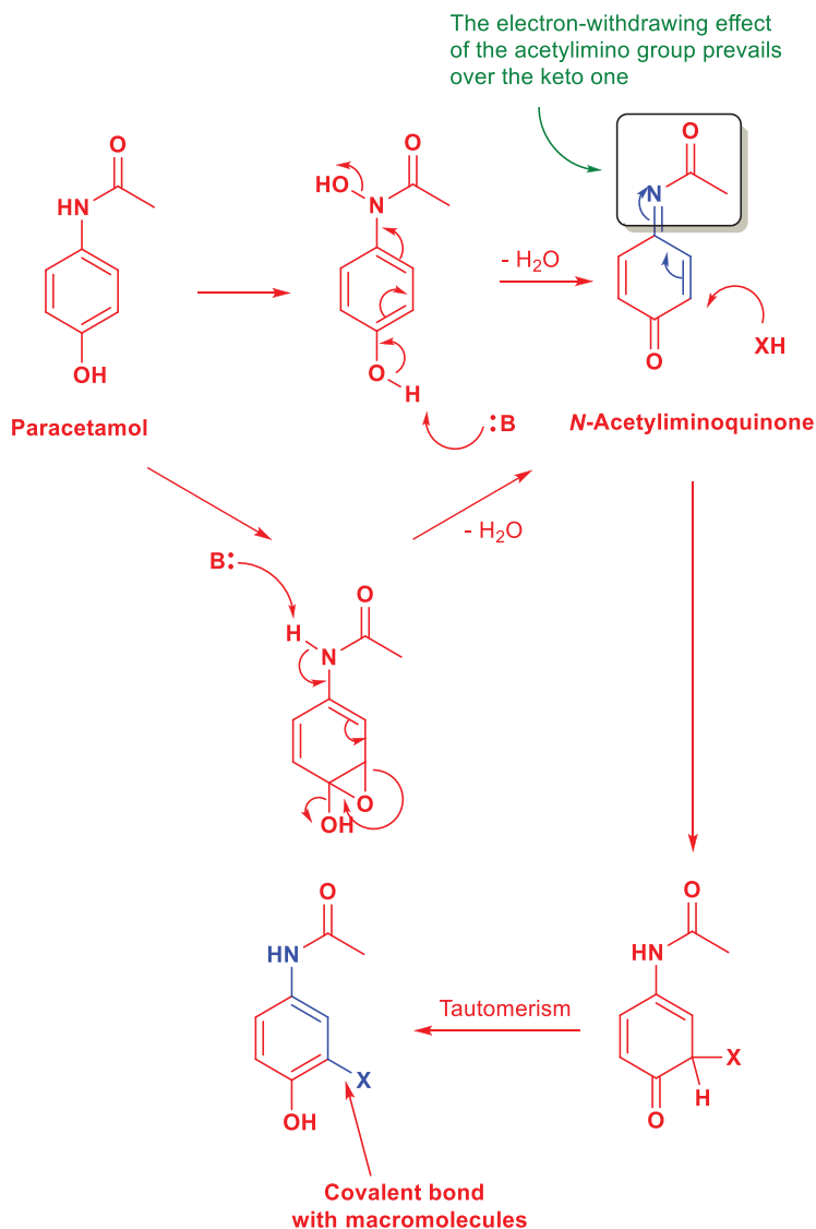
Scheme 7.18: Formation of iminoquinones (possible cytotoxic agents) in the oxidative metabolism of paracetamol.
