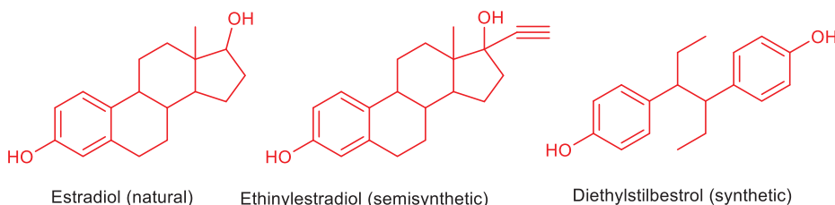
Fig. 1.5: Examples of natural, semisynthetic, and synthetic drugs.
