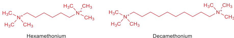
Fig. 4.15: An example of homologous derivatives.
