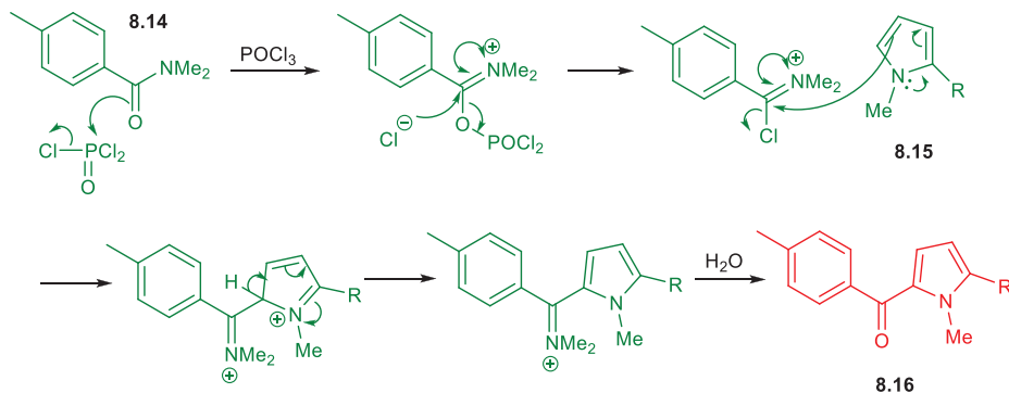
Scheme 8.25: Application of the Vilsmeier acylation on N -methylpyrrole.
