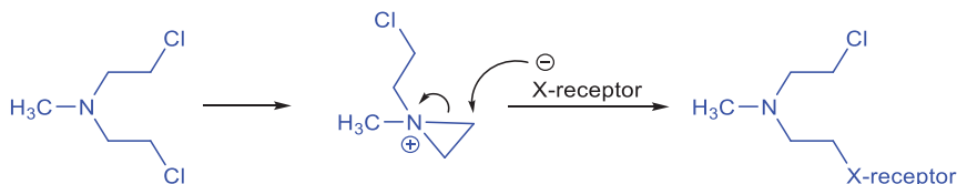
Fig. 5.11: Formation of an irreversible covalent bond.
