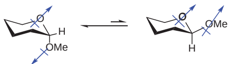
Fig. 7.12: A second interpretation of the anomeric effect.
