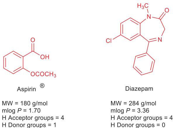
Fig. 7.3: Lipinski's rules applied to Aspirin ® and diazepam.
