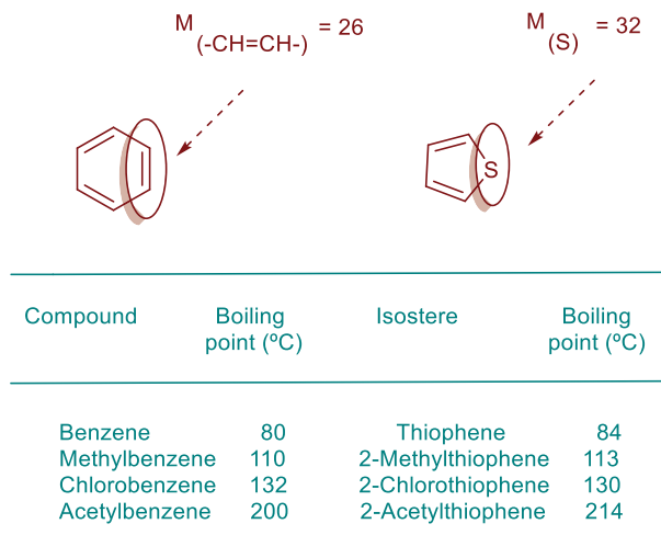
Fig. 4.21: Similarity of boiling points among several benzene and thiophene derivatives.
