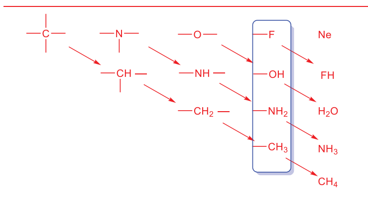
Fig. 4.19: Grimm's hydride displacement law. In each vertical column, the atom is followed by its pseudoatom.
