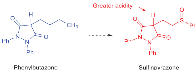
Fig. 4.6: Sulfinpyrazone has a higher uricosuric activity than phenylbutazone.
