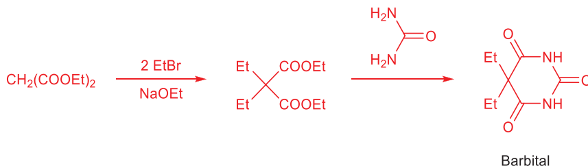
Scheme 8.1: Synthesis of barbital.
