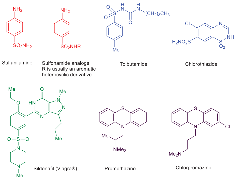
Fig. 3.6: Drugs developed through potentiation of a side effect.
