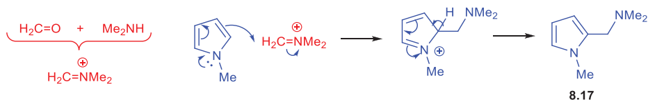
Scheme 8.26: Synthesis of N,N -dimethyl-1-(1-methyl-1 H -pyrrole-2-yl)methanamine.
