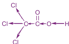
Fig. 6.5: Trichloroacetic acid (TCA) is a strong acid: from a chemical ionization point of view, TCA is a much stronger acid than acetic acid because electronegative chlorine atoms remove electron density from the carboxyl end of the molecule, producing a partial positive charge on the carboxyl moiety.
